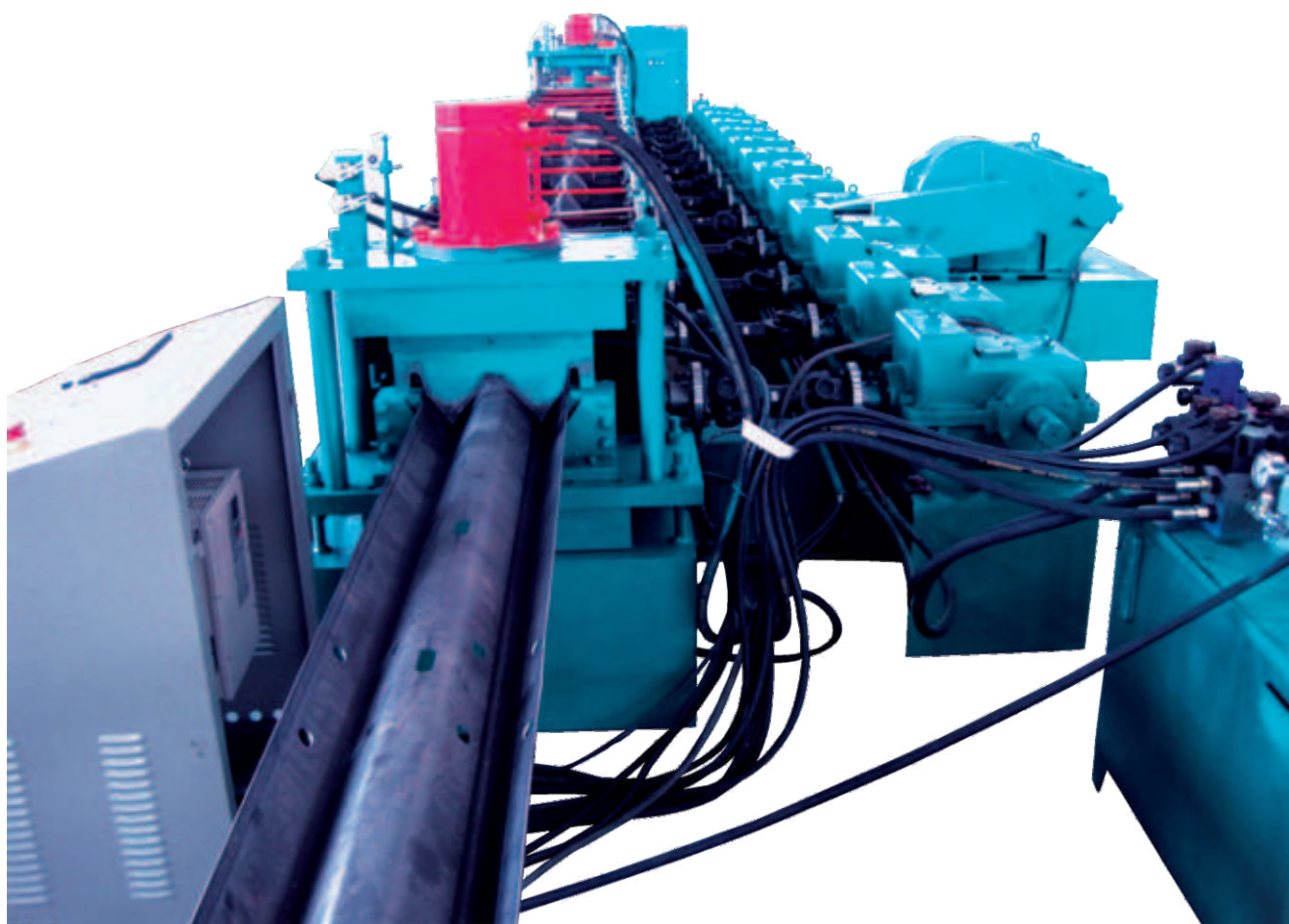
GUARDRAIL ROLL FORMING MACHINE
