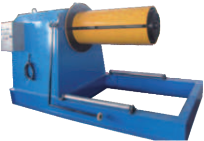
10T Hydraulic Uncoiler
