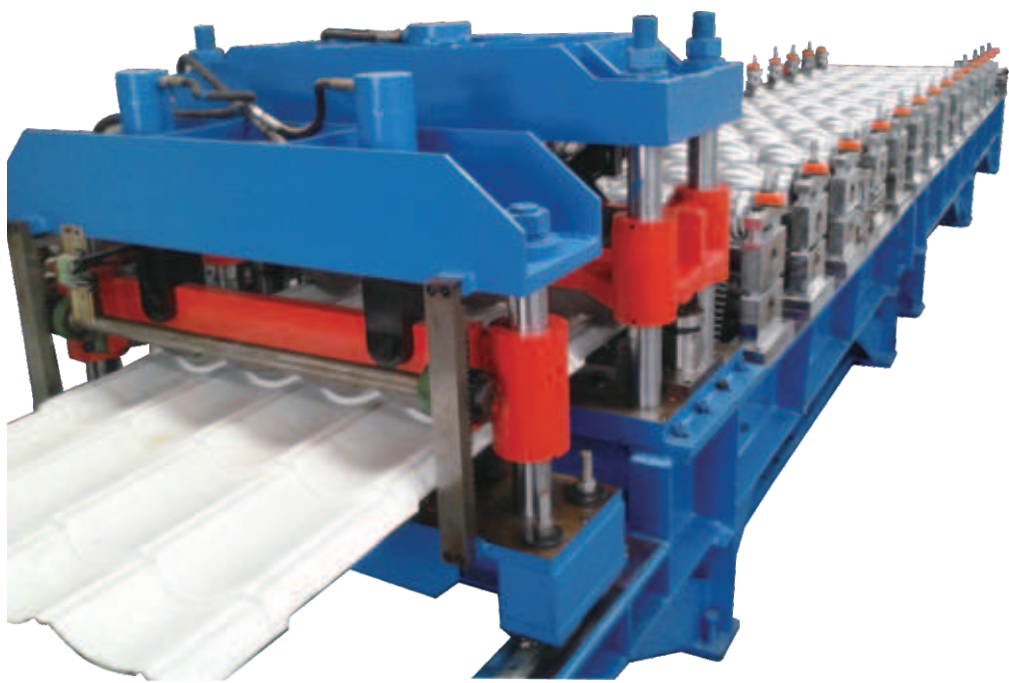
CLOUMN STATION CORRUGATED TILE MACHINE
