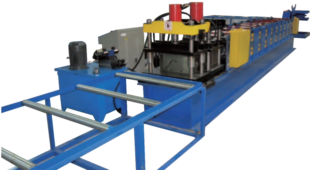
RIDGE CAP ROLL FORMING MACHINE
