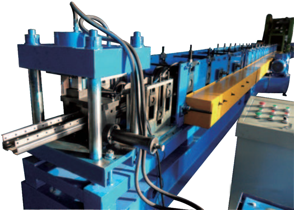
RACK ROLL FORMING MACHINE
